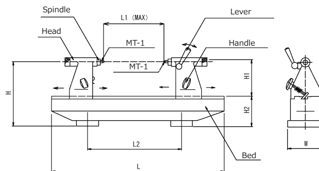
■ Dimensional drawing Unit : mm
