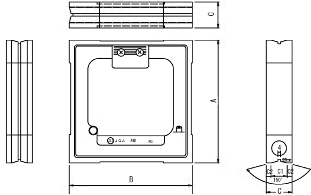
■ Dimensional drawing Unit : mm
