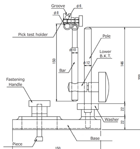
Dial stand for P-type pick testing
